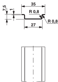
Dimensional drawing
